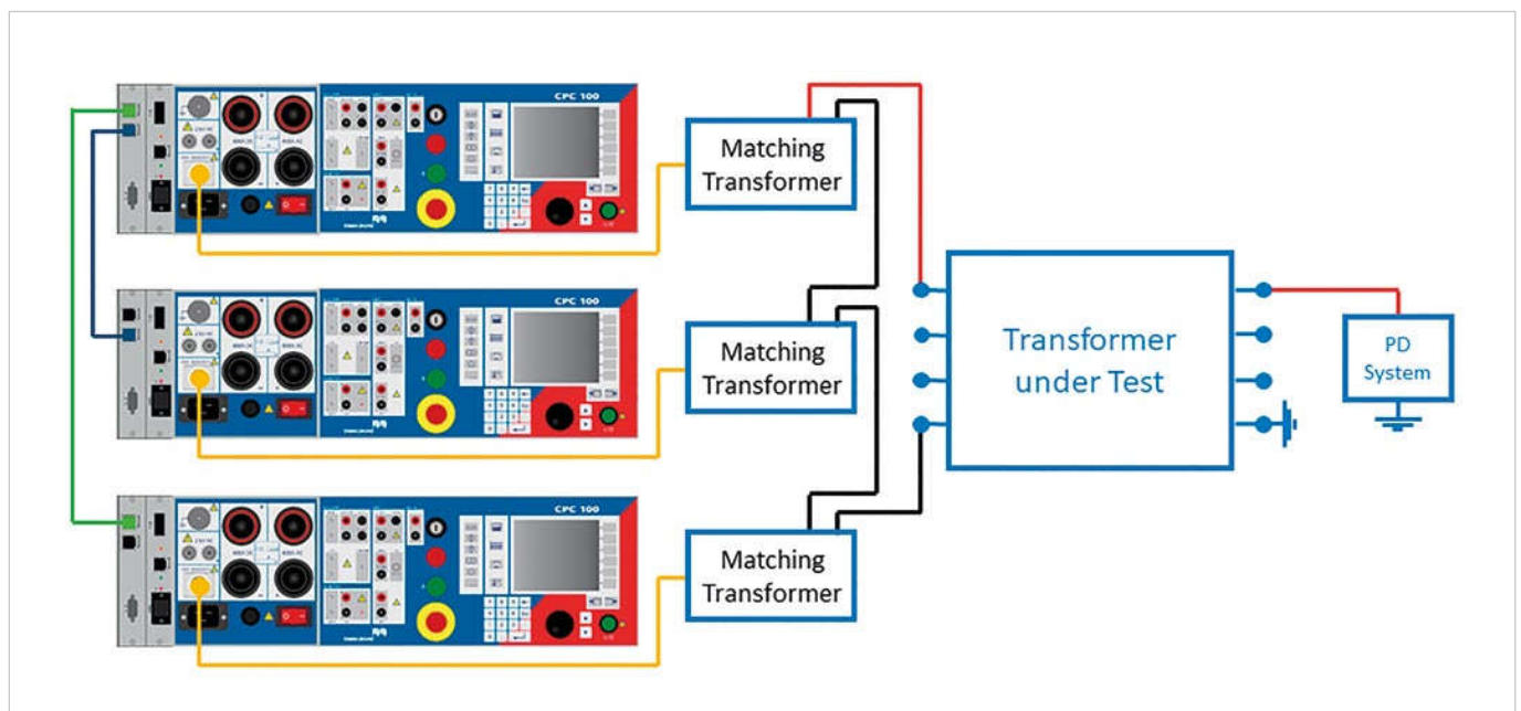
Figure 3. Test system for 15 kVA with three CPC 100
