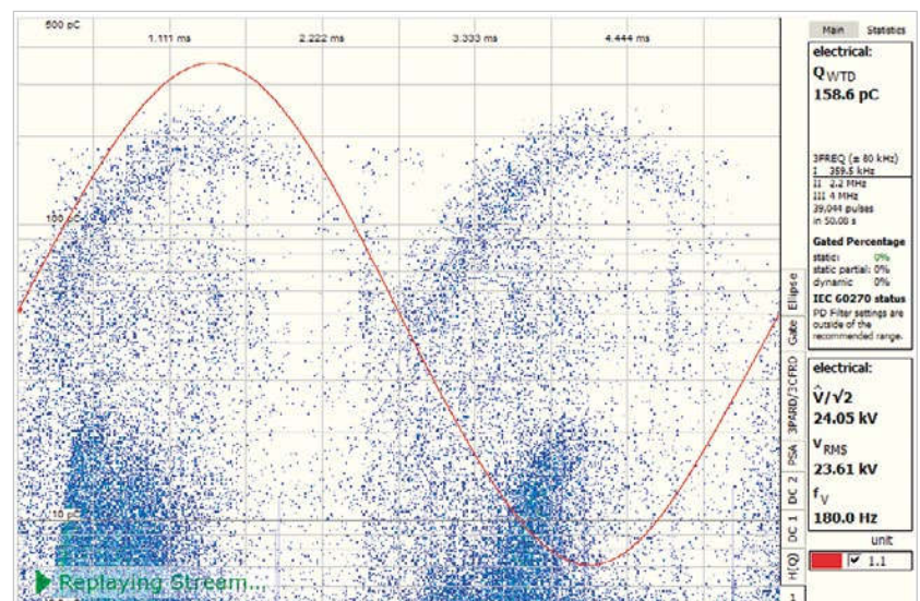
Figure 10. PD measurement results
