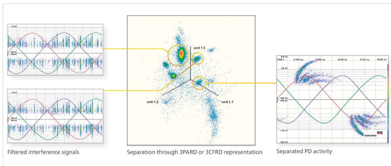
Figure 5. Separation through 3PARD or 3CFRD representation
