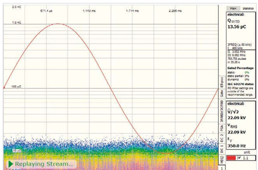
Figure 12. PD measurement results on phase B
