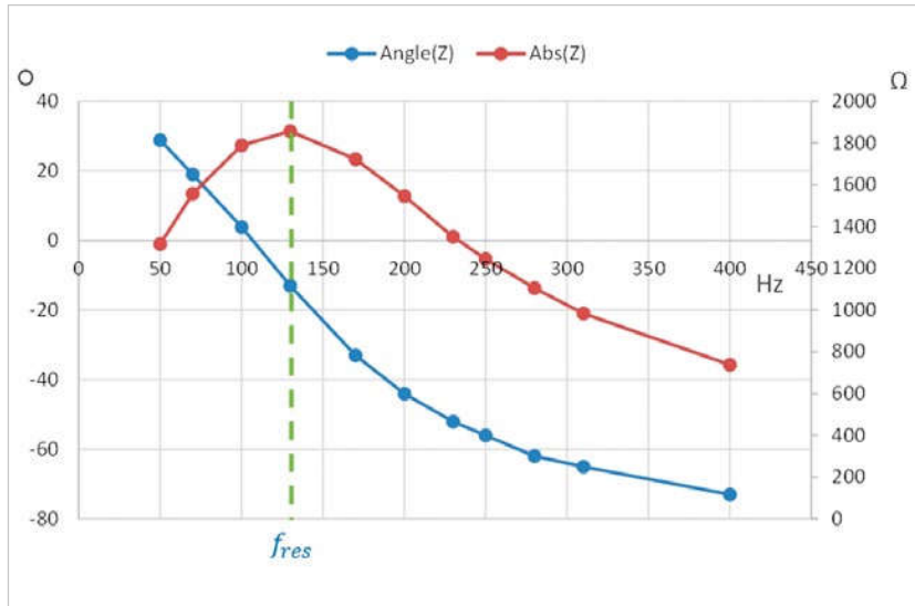
Figure 2. Impedance of the test circuit vs. frequency
