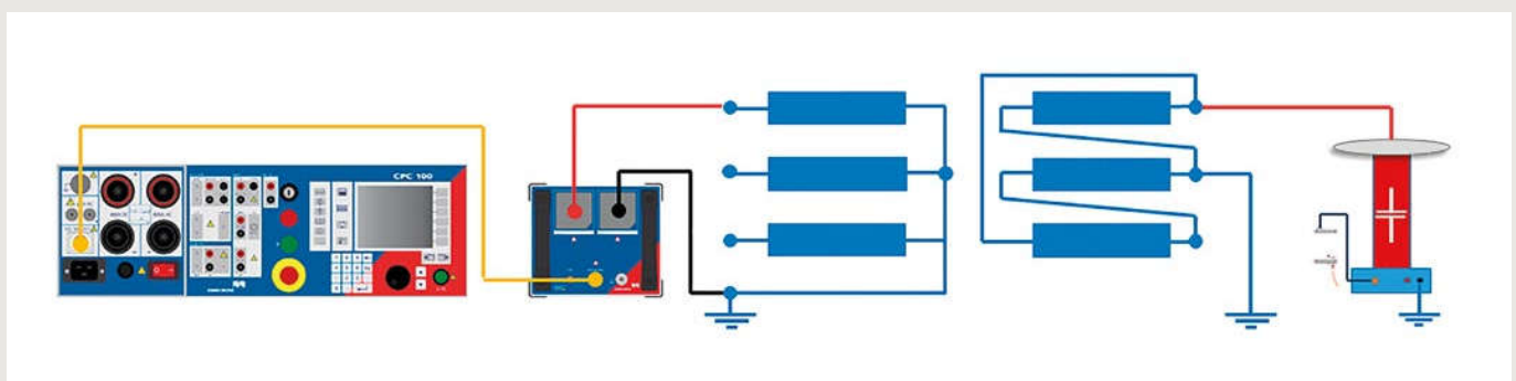
Figure 1. CPC 100 with matching transformers
