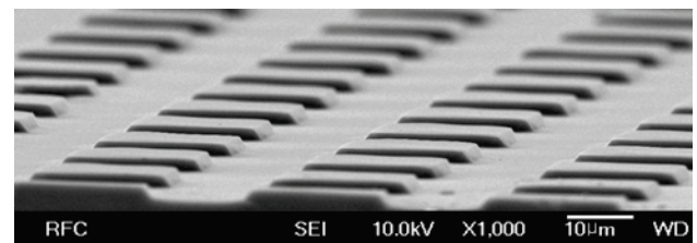
Figure 1 SEM image of modified PDMS
