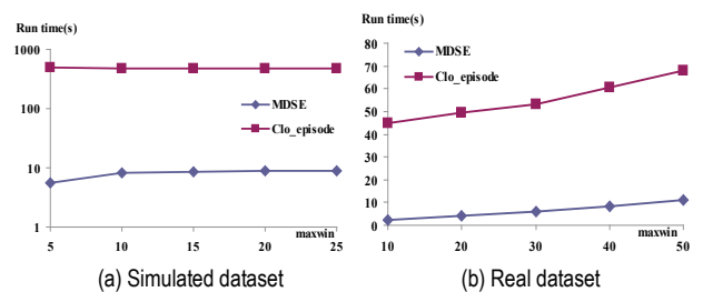
Figure 6 The running time comparison under different time window sizes
