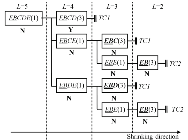
Figure 3 The shrinking example of EBCDE
