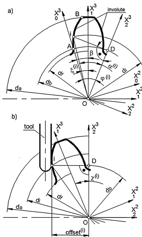
Figure 6 Schematic diagram of tool positioning for Cv-Cc tooth machining
