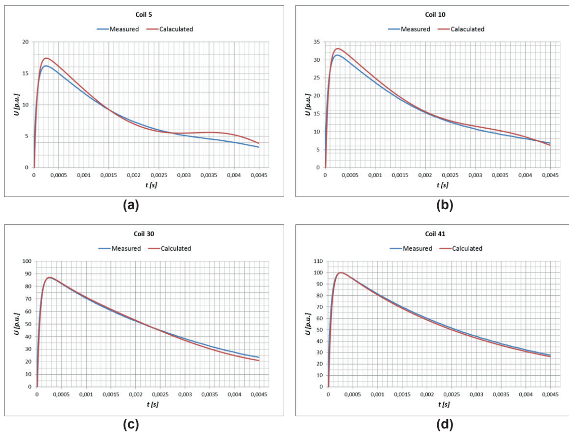
Figure 10 - Comparison of switching impulse voltage distribution (a) Coil 5 (b) Coil 10 (c) Coil 30 (d) Coil 41
