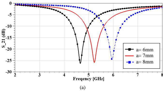
Fig. 3. Variation of the transmission coefficient (a) length (b) width (c) gap width (d) slot width simulated with HFSS.
