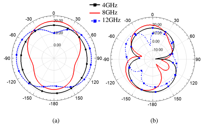
Fig. 9. Radiation pattern : (a) H-plane (b) E-plane simulated with HFSS.
