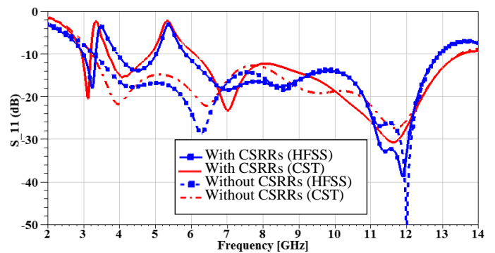
Fig. 5. S (11) parameter of the proposed dual band notched antenna and the reference antenna.
