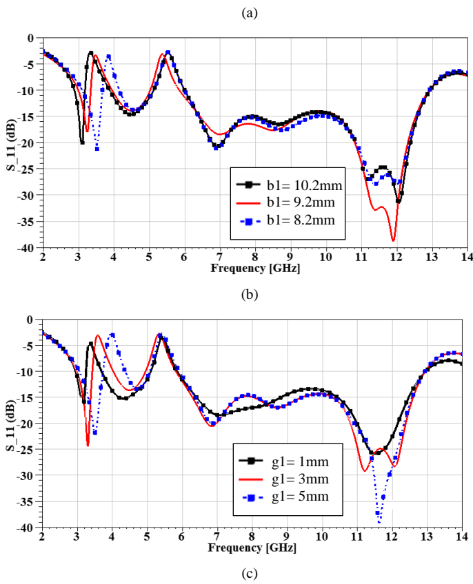
Fig. 6. S_{11} parameter for various : (a) length a_1 , (b) width b_1 and (c) gap width g_1 , simulated with HFSS.
