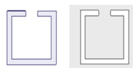
Fig. 1. Topology of the (a) Single SRR, (b) Single CSRR (Metal regions are depicted in gray).
