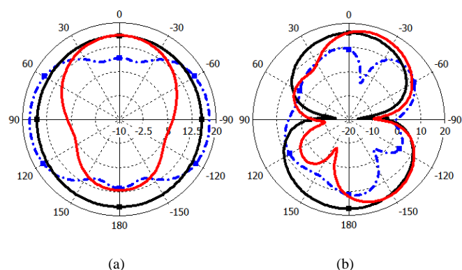
Fig. 10. Radiation pattern: (a) H-plane (b) E-plane simulated with CST.
