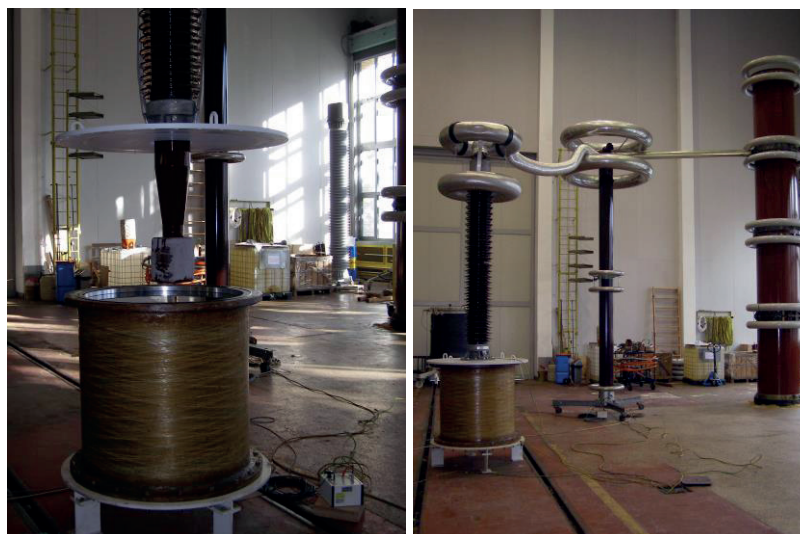
Figure 11. Screen electrode test setup
