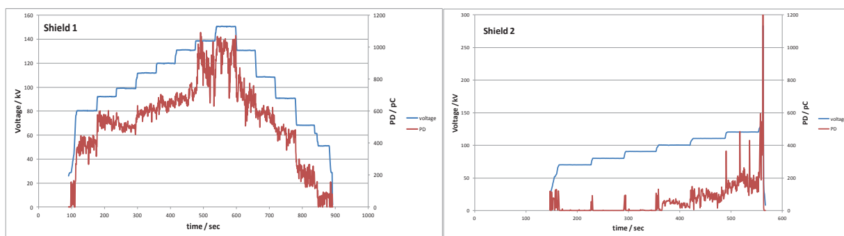
Figure 12. Plot of voltage and PD level vs. test time
