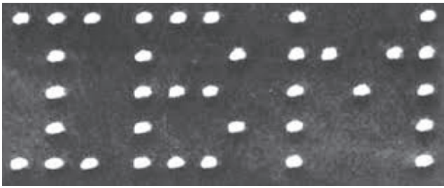
Figure 2. "IBM" formed by means of 35 xenon atoms, [7]
