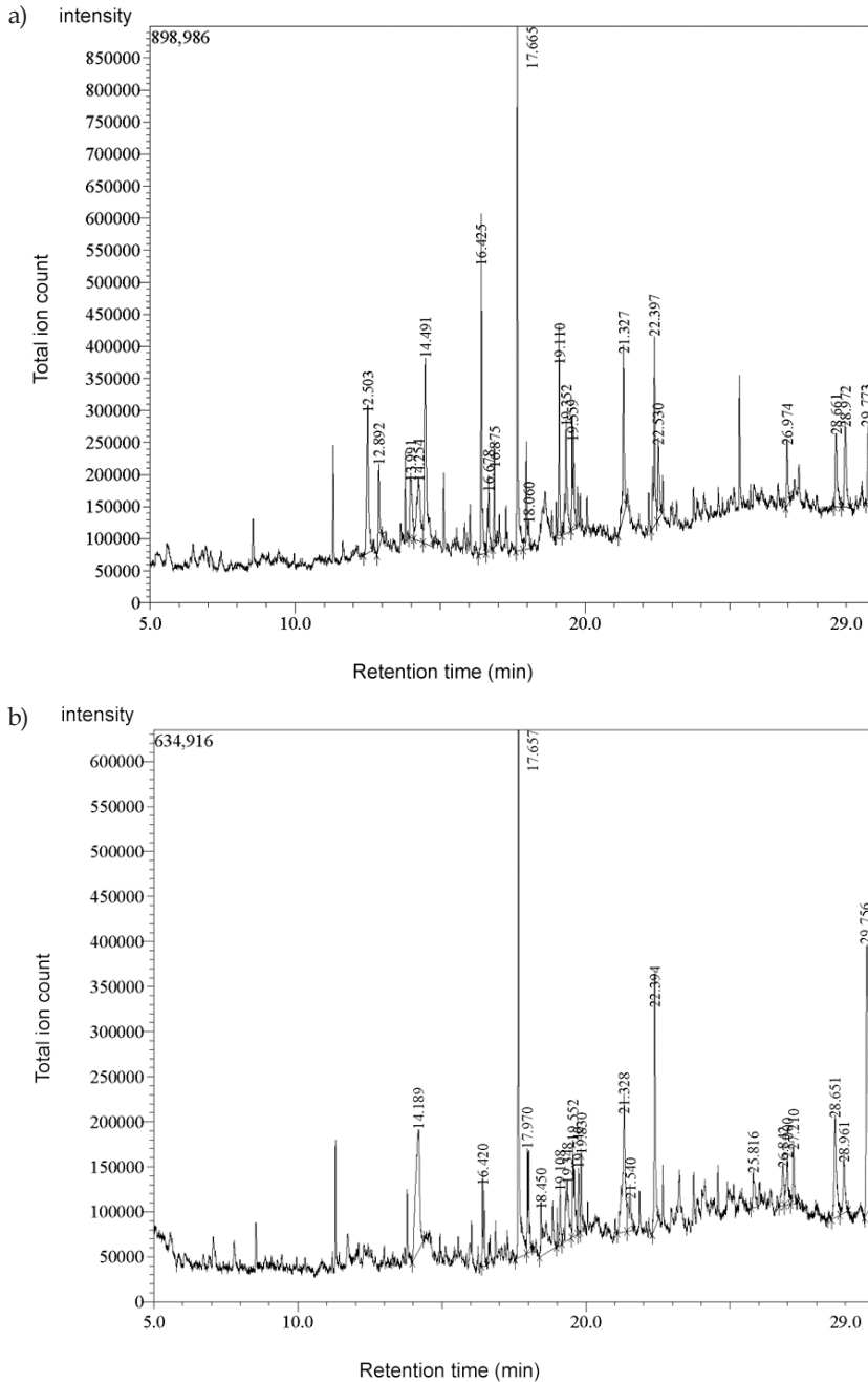
Fig. 3. GC-MS chromatograms of ethanolic extracts of A. wilkesiana : a) leaves, b), stem bark and c) root bark.
