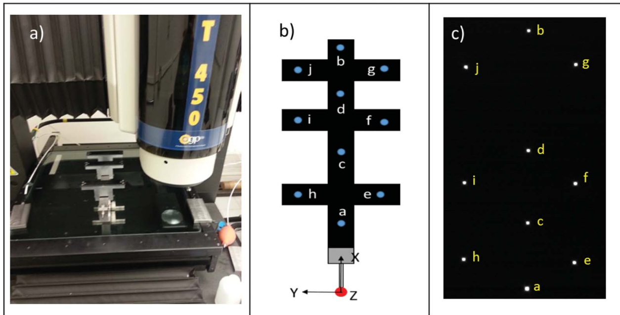
Figure 5. (a) OCMM calibrating each LED and spherical probe tip position of the hand tool. (b) Local coordinate system of the hand tool with labelled infrared LEDs. (c) Image of infrared LEDs viewed by the camera and tracked-ordered with Algorithm 1.
