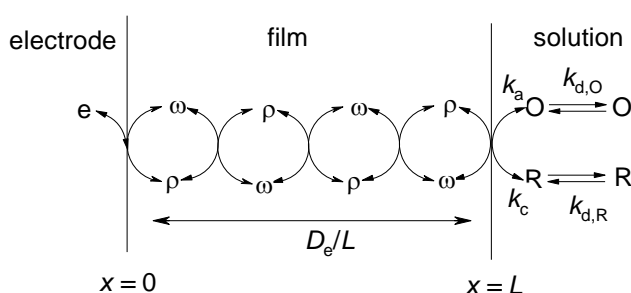
Figure 1. Schematic representation of the mediation process in redox polymer coated electrodes.
