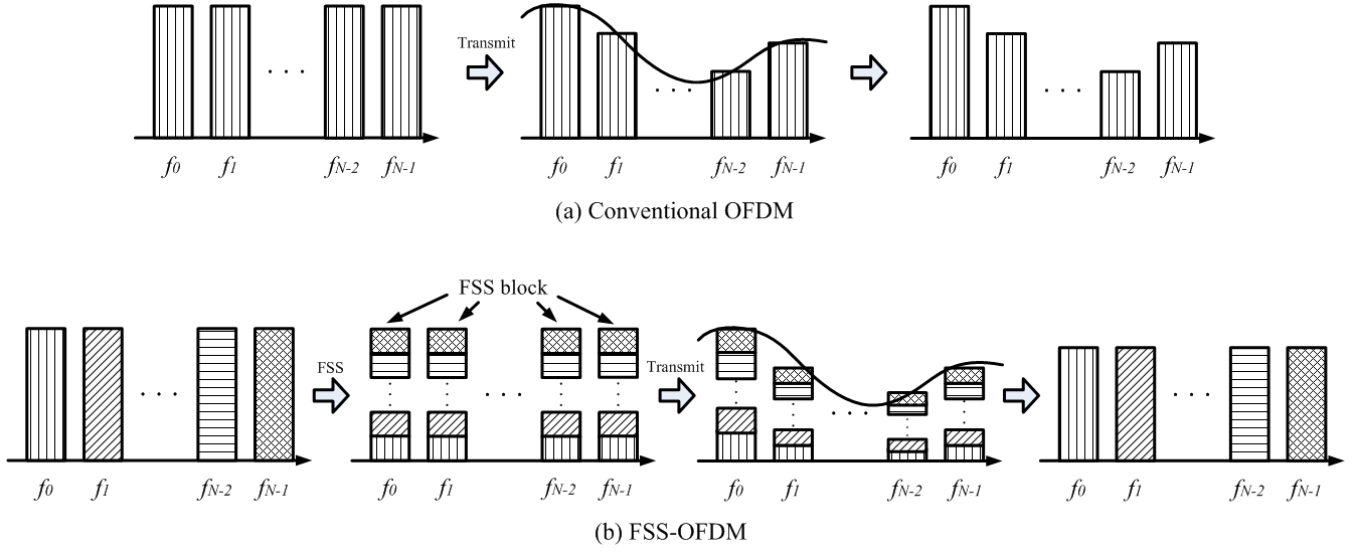
Fig. 1. A concept of FSS.
