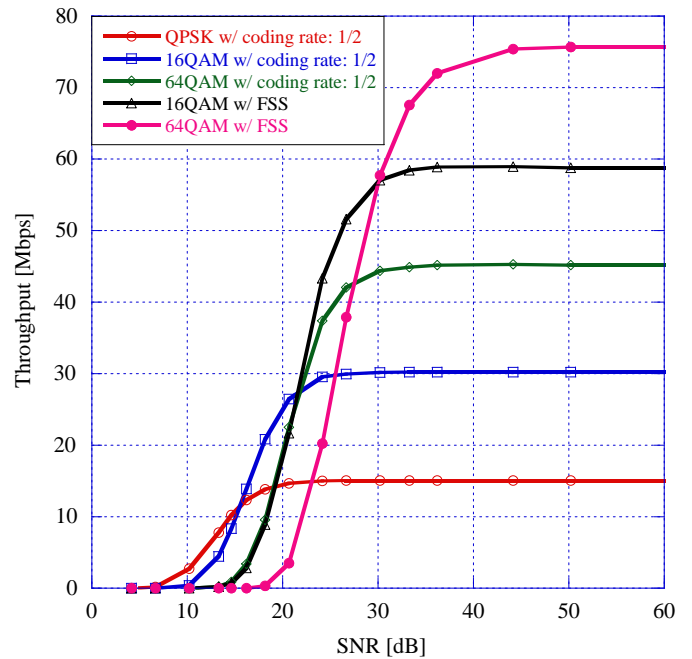
Fig. 9. Throughput performance at Doppler frequency of 40 Hz.
