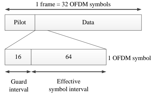
Fig. 3. Frame structure.
