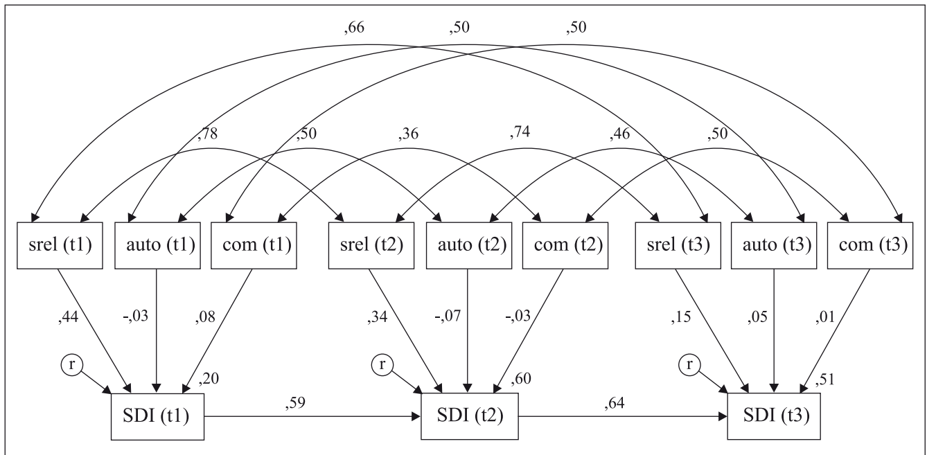
Figure 6. Path diagram with SDI and basic needs
