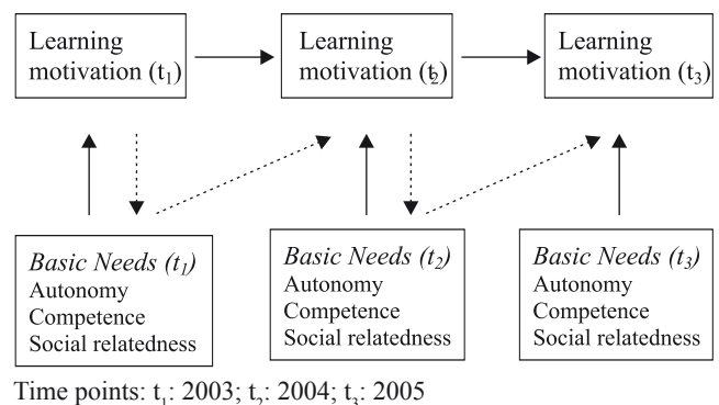
Figure 2. Design of the longitudinal analysis
