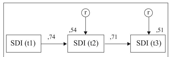
Figure 4. Path diagram for self-determination index (SDI) ( t_1 - t_3 )
