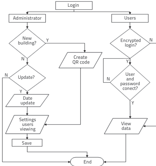
Figure 7. Algorithm for software system
