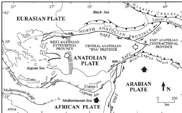
Figure 2. Tectonic map of Turkey with major structural features [57]
