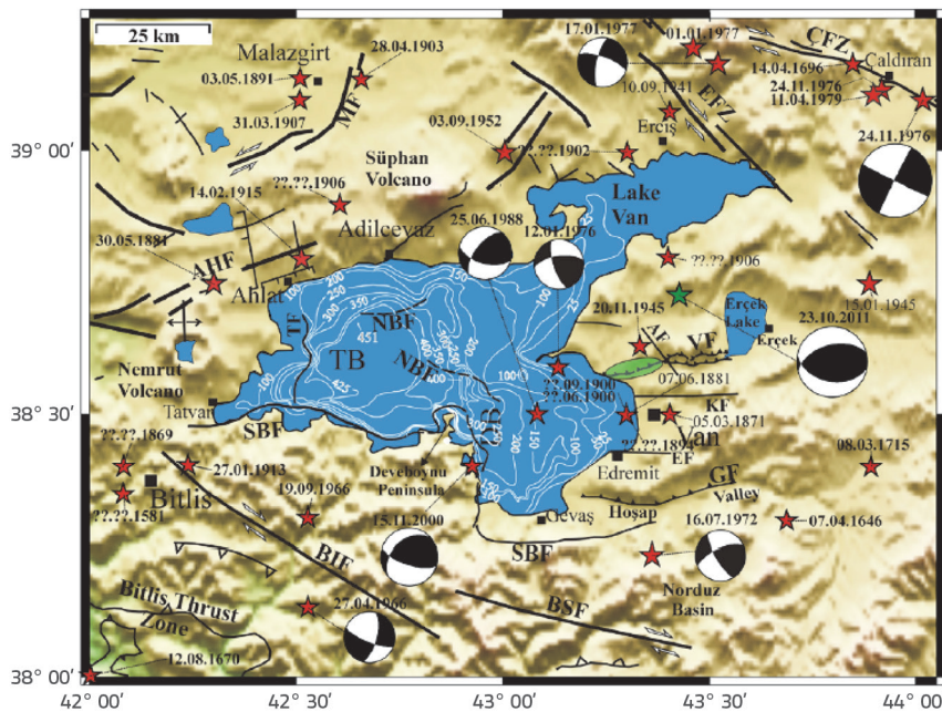
Figure 3. Significant tectonic structures of Van Lake Basin [59]
