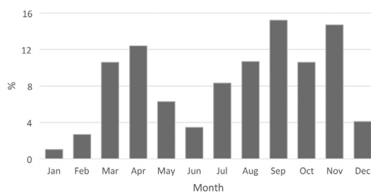
Fig. 1. Proportion of total monthly catches in overall catches for whole investigated period (2013-2016) obtained with purse seine “Srdelara” by involved commercial vessel (PS), all purse seiners fishing in fishing zone G (PS_G) and all purse seiners fishing in whole Croatian fishing ground (PS_ALL)
