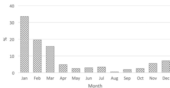
Fig. 2. Average monthly appearance of three predators – tuna (a), dolphins (b), swordfish (c) that accompany purse seine fishing activity in fishing zone G, Adriatic, 2013-2016
