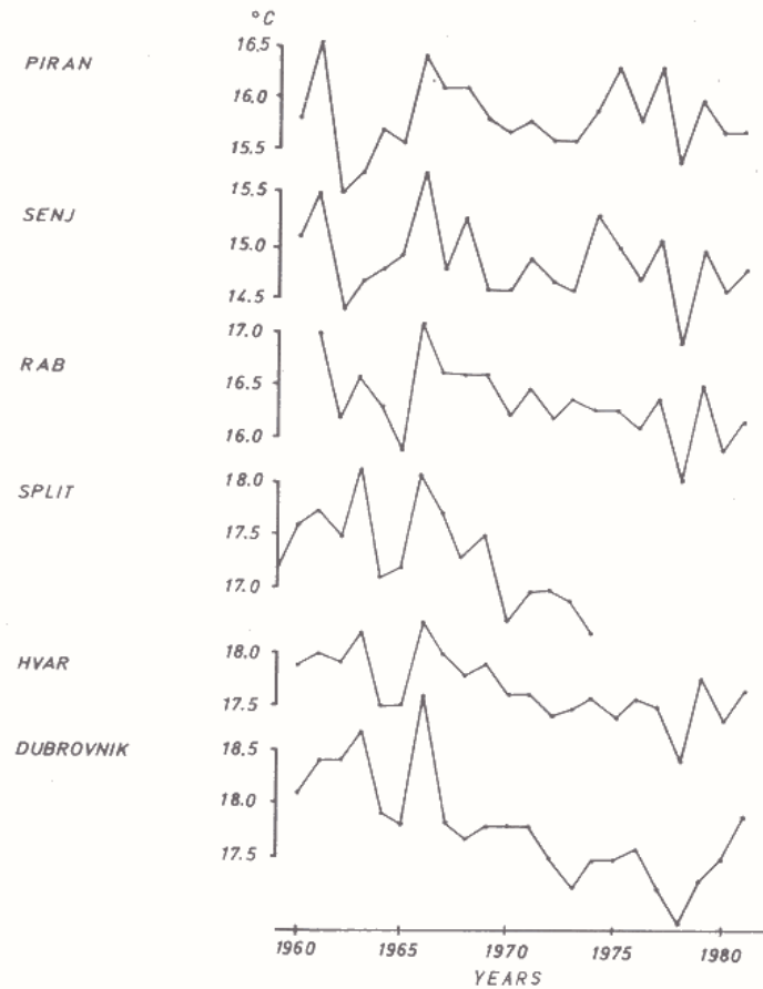
Figure 6. Year-to-year variability of the mean annual SST at six stations.
