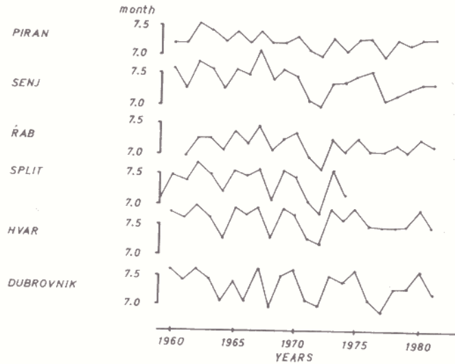
Figure 9. Interannual variability of phases of the first harmonic of the SST annual cycle at six stations.
