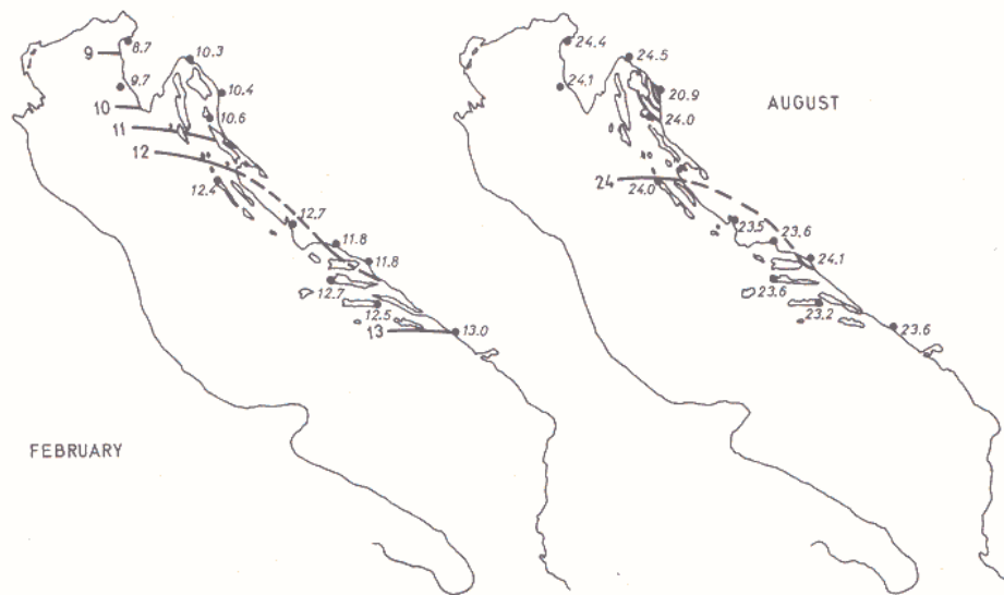
Figure 4. Spatial distribution of SSTs, averaged for February (left) and August (right) over a 5-year interval (1970-74).
