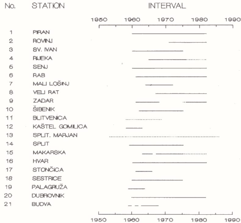
Figure 2. Intervals for which data were available at stations indicated in Figure 1. Solid lines represent intervals over which measurements were performed three times a day, dotted lines mark intervals with only two readings made per day.
