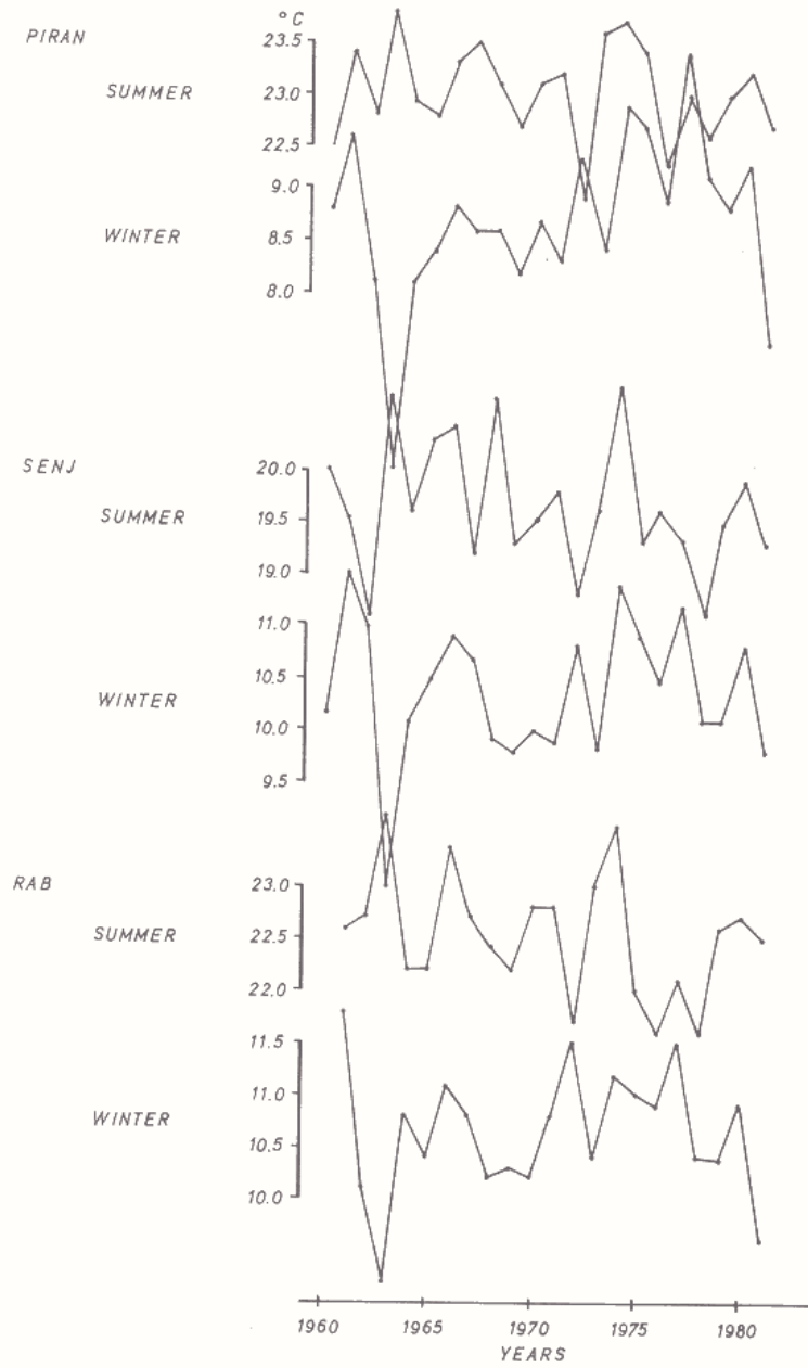
Figure 8a. Time series of the average summer (July, August, September) and winter (January, February, March) temperatures at stations Piran, Senj and Rab.
