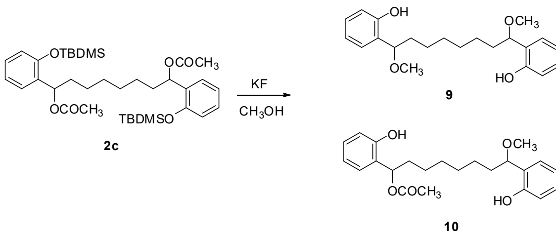
Scheme 4. F^- induced methanolysis from bisphenol 2c .
