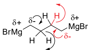
Figure 2. Structure of C-4 di-Grignard reagent that is prone to \beta -hydride transfer.
