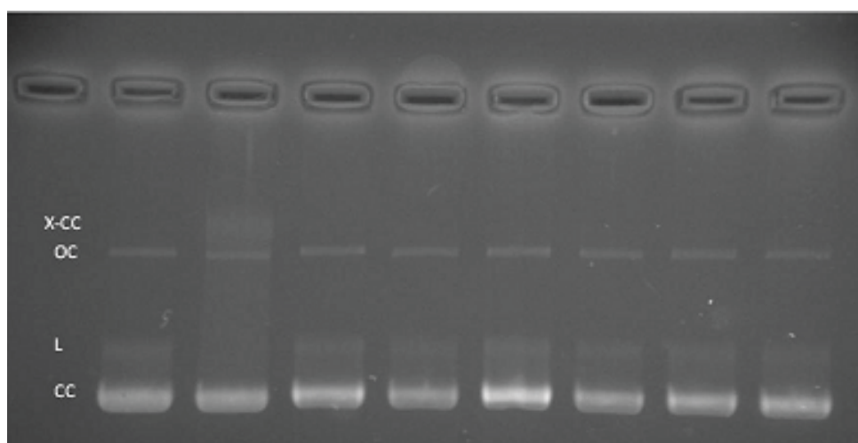
Figure 4. Alkaline agarose gel electrophoresis: pCMVbeta plasmid DNA (2 \mu g) in PBS buffer ( pH = 7.4 ) was mixed with 2a–2e or 7 (1 mM), and KF (200 mM). After 18 h incubation, the samples were loaded and the gel was running for 5 h. Columns from left to right: 1) plasmid DNA, 2) psoralen (PS) (20 \mu M) and irradiation 5 min at 300 nm, 3) 2a 4) 2b , 5) 2c , 6) 2d , 7) 2e , 8) 7 . CC-closed circular DNA, OC-open circular DNA, L-linear DNA, X- cross-linked DNA.
