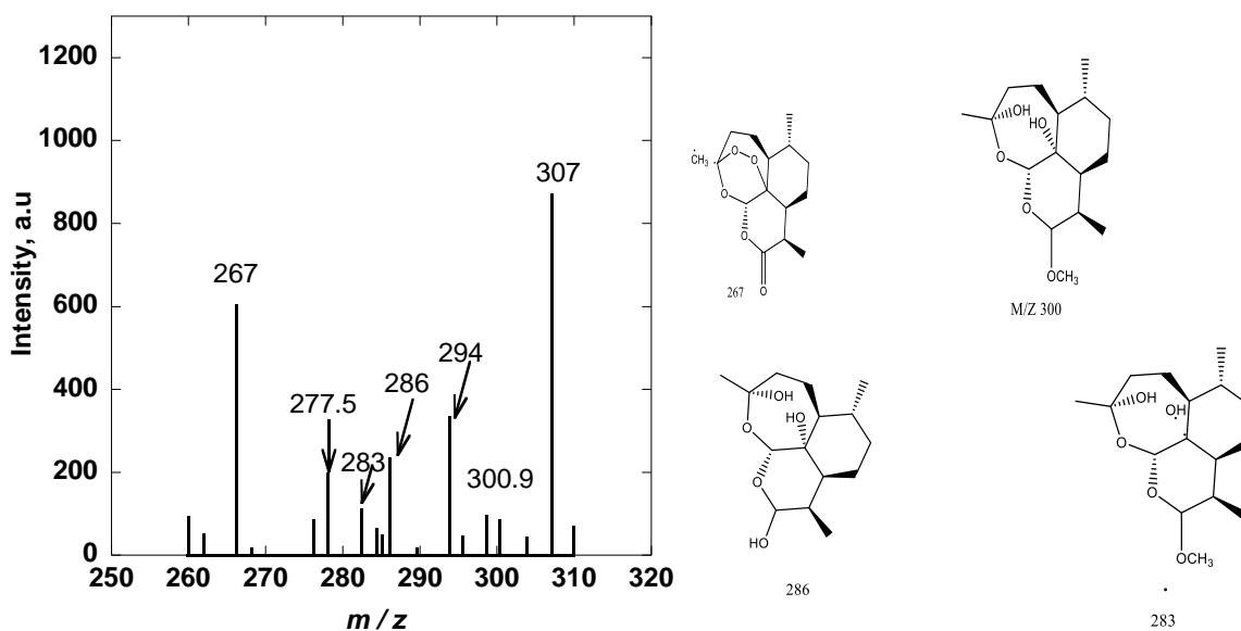
Figure 9. Mass spectrum of ART after three hours of electrolysis (peak at 21.5)
