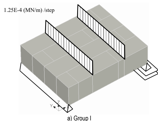
Figure 5 Micromodel composition
