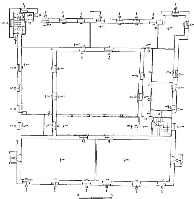
Kaštel Vitturi, tlocrt 2. kata (Konzervatorski odjel Split) Castle Vitturi, second floor layout
