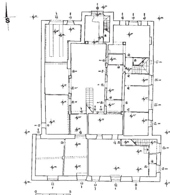
Kaštel Cippico u Kaštel Starom, tlocrt prizemlja (Konzervatorski odjel Split) Castle Cippico in Kaštel Stari, ground floor layout
