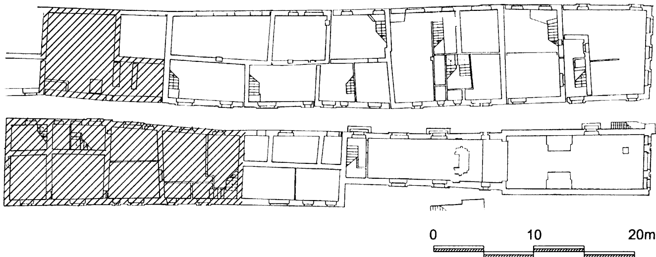
Trogir, Macanovića dvori, tlocrt prizemlja, planoteka Konzervatorskog zavoda u Splitu Trogir, Macanović Hall, first-floor layout
