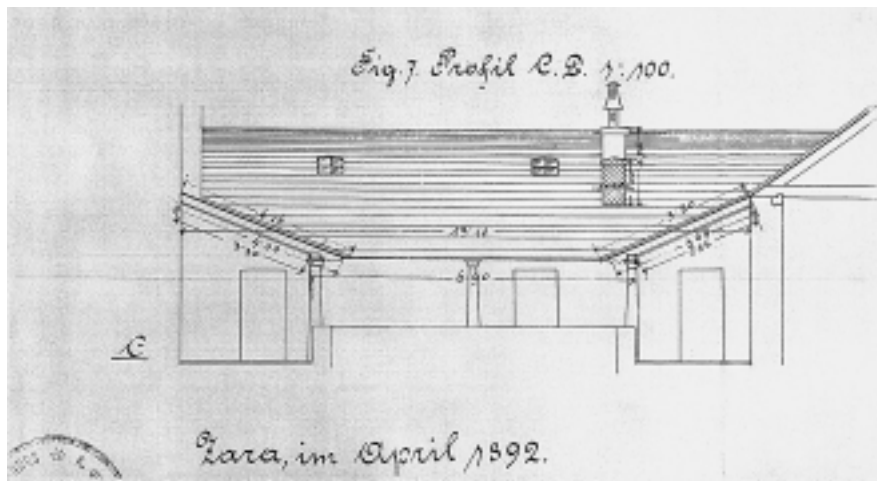
Presjek drugoga kata trijema samostana Sv. Marcele, nacrt izrađen 1892. god. Second floor section of the monastery cloister of St. Marcela, plan made in 1892
