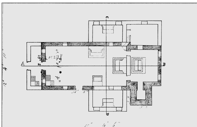
Nacrt za proširenje crkve Gospe od Ružarija u Preku Design for Extension of the Church of Our Lady of the Rosary in Preko
