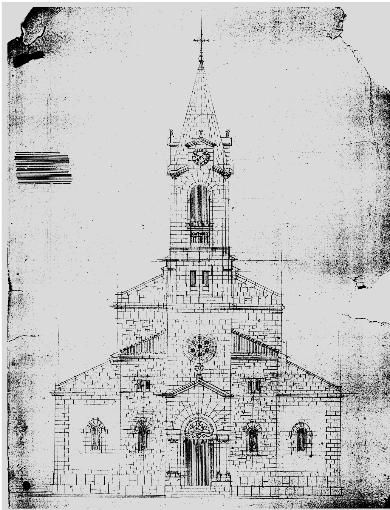
Ivekovićev nacrt za novu crkvu Gospe od Ružarija u Preku Iveković's Design for the New Church of Our Lady of the Rosary in Preko
