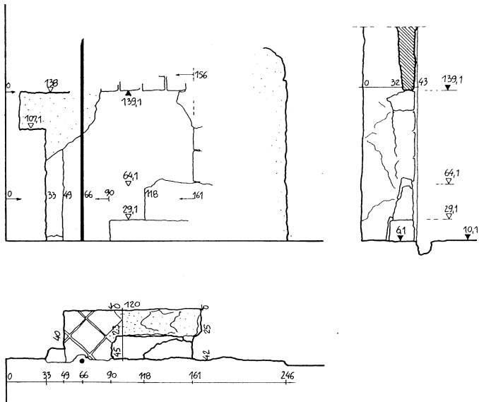
12. Kamin u bočnoj sobi kata (prostoriya 3, snimio Nikola Nađ) 12. Fireplace in a lateral room on the first floor (room 3, drawing Nikola Nađ)
