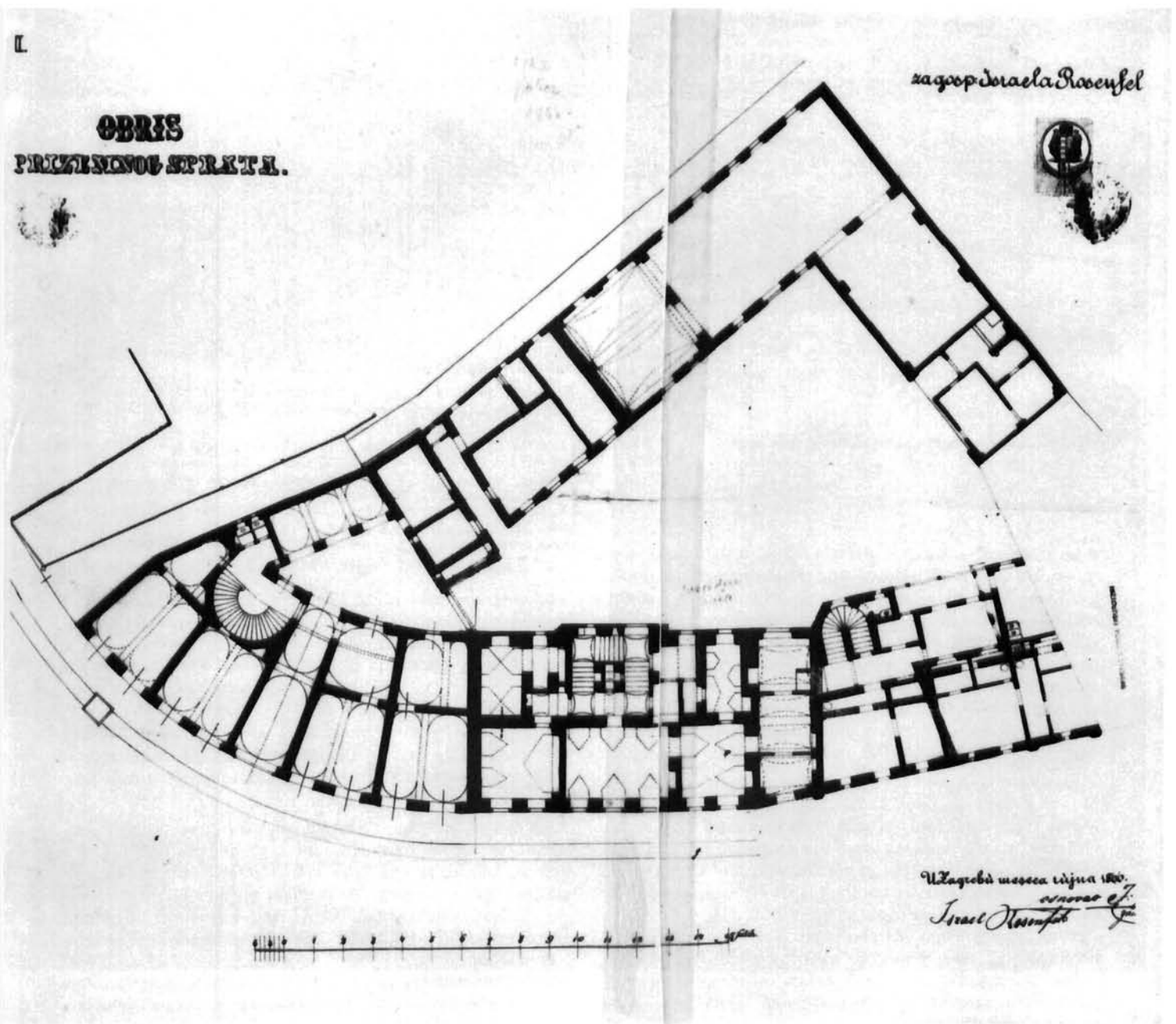
N. Grahor: Tlocrti prizemlja kuća u Mesničkoj 1, 3 i 5 (1866.) (Muzej grada Zagreba) N. Grahor: plans of the ground floor of the houses at Mesnička Street 1, 3 and 5 (1866). Zagreb Municipal Museum
