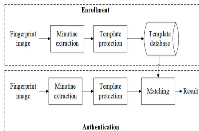
Figure 1 Fingerprint-based authentication system with a template protection
