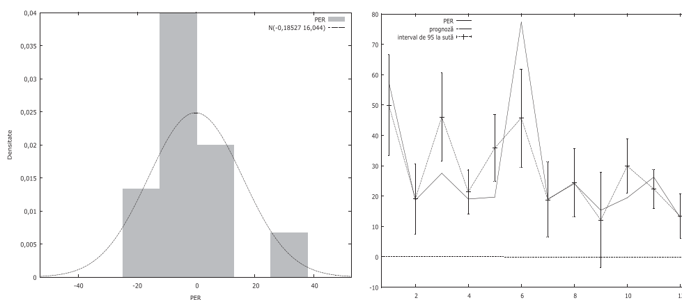
Figure 1. (a) Histogram of errors (b) forecast chart. Source: GRETL program, the 2019d version.
