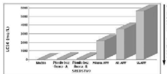
Slika 6. Test LC 50 (96 h) na juvenilnoj pastrvi (32) Figure 6. Test LC 50 (96 h) on juvenile California trout
