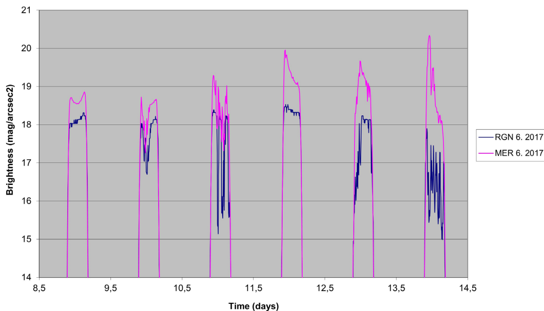
Figure 3: An enlarged part of the graph in Figure 2 showing night sky brightness patterns at both sites in more detail. In most cases, the patterns are very similar. A more pronounced difference is evident in the last night (14-15th) on the graph. Note that the influence of the Moon is more pronounced at the Merenje site, as the light pollution there is lower, thus the moonlight alone makes a larger contribution to the night sky brightness, when the Moon is up. In this case, the Moon was up almost the whole night, as the Moon was full on June 9th.
