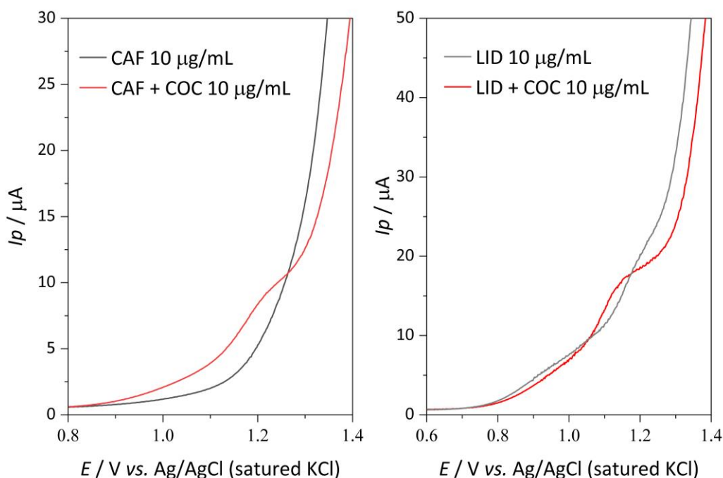
Figure 6. SW voltammograms of two main cocaine adulterants: (a) black voltammogram represents 10 \mu\text{g}/\text{mL} caffeine, and red voltammogram represents 10 \mu\text{g}/\text{mL} caffeine with addition of 10 \mu\text{g}/\text{mL} freebase cocaine (1:1). (b) black voltammogram represents 10 \mu\text{g}/\text{mL} lidocaine, and red voltammogram represents 10 \mu\text{g}/\text{mL} lidocaine with addition of 10 \mu\text{g}/\text{mL} freebase cocaine (1:1). Supporting electrolyte: 0.1 mol/L \text{NH}_4\text{ClO}_4 with 0.1 mol/L \text{K}_2\text{HPO}_4 , pH 9.5. SWV experimental parameters are given in Table 1
