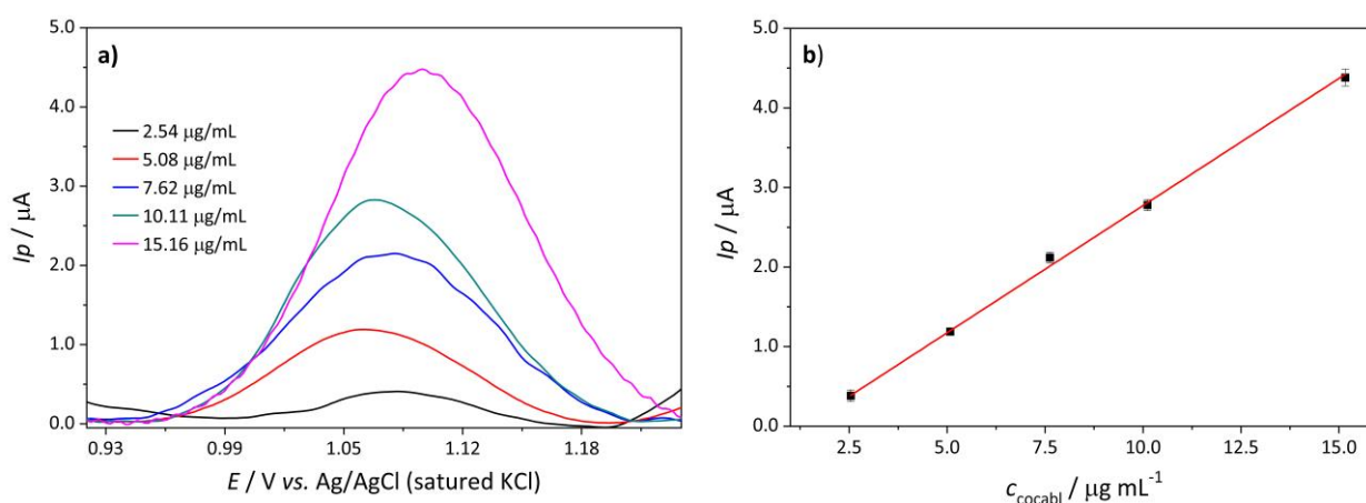
Figure 5. (a) SW voltammograms of freebase cocaine (concentrations: 2.54, 5.08, 7.62, 10.11, and 15.16 \mu\text{g/mL} ) in the supporting electrolyte (0.1 mol/L \text{NH}_4\text{ClO}_4 and 0.1 mol/L \text{K}_2\text{HPO}_4 , pH 9.5) and (b) relation between peak current and concentration of freebase cocaine.
