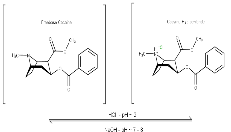
Figure 1. Molecular structure difference between freebase cocaine and cocaine hydrochloride.
