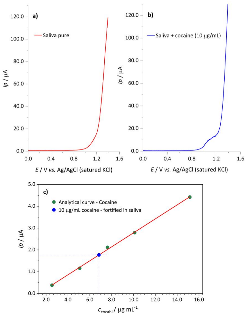
Figure 8. SW voltammograms of (a) pure artificial saliva and (b) artificial saliva containing 10 µg/mL of freebase cocaine. (c) Anodic peak current of 10 µg/mL freebase cocaine (1.77 µA) is denoted as blue point in the analytical curve of freebase cocaine. Supporting electrolyte: 0.1 mol/L \text{NH}_4\text{ClO}_4 and 0.1 mol/L \text{K}_2\text{HPO}_4 , pH 9.5. SWV experimental parameters are given in Table 1
