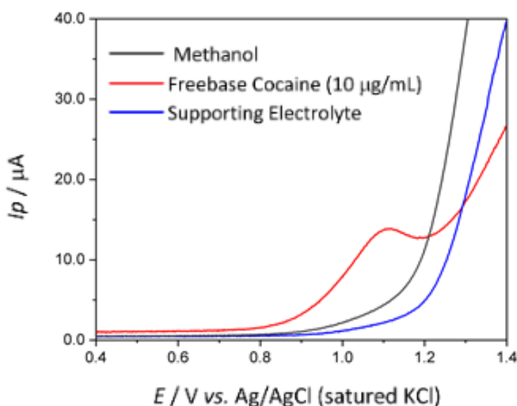
Figure 4. Screening of freebase cocaine ( 10 \mu\text{g/mL} ) detection on carbon paste electrode using SWV in 0.1 \text{ mol/L NH}_4\text{ClO}_4 and 0.1 \text{ mol/L K}_2\text{HPO}_4 as supporting electrolyte (red). SW voltammograms of 40 \mu\text{L} pure methanol (black) and pure supporting electrolyte (blue). Experimental SWV parameters: f=100 \text{ Hz} , A = 0.010 \text{ V} , pre-concentration time of 60 \text{ s} at 1.0 \text{ V} .
