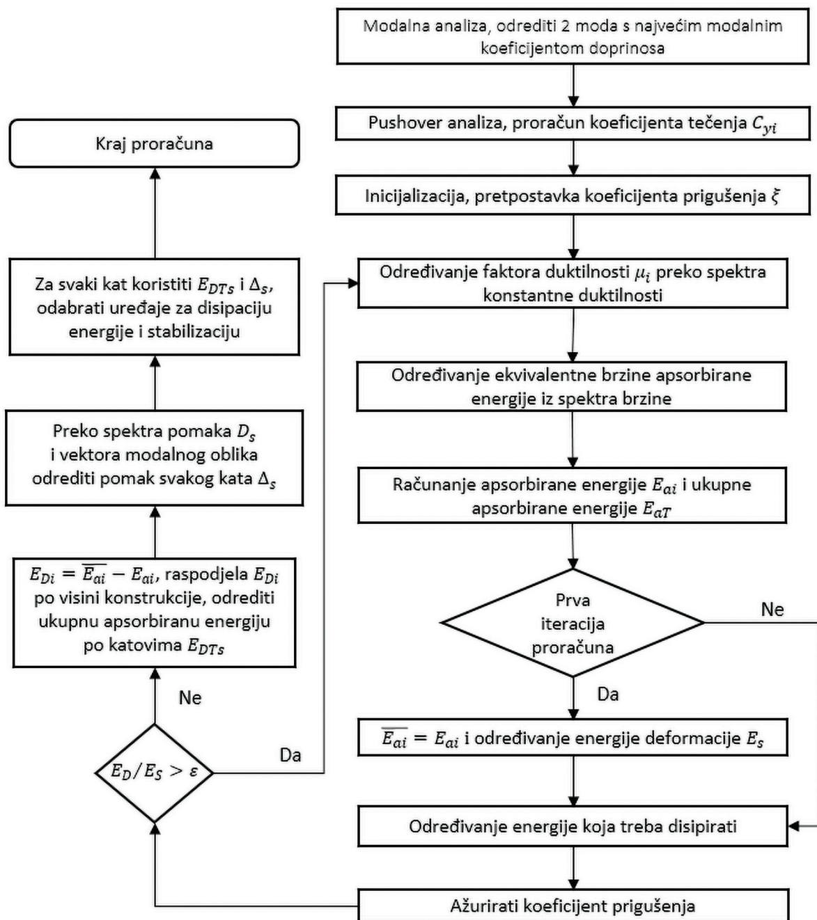
Slika 10 Dijagram toka energetske metode za seizmička ojačanja s pasivnim energetskim disipatorima [24] Figure 10 The flowchart for a energy-based design with passive energy dissipators proposed by [24]
