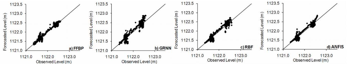
Figure 10. Scatter plot for the testing data at 30 days ahead estimation case for (a) FFBP, (b) GRNN, (c) RBF, and (d) ANFIS
