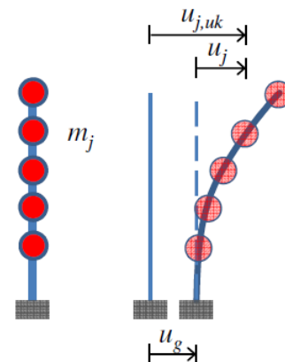
Figure 2. Multi-degree system
