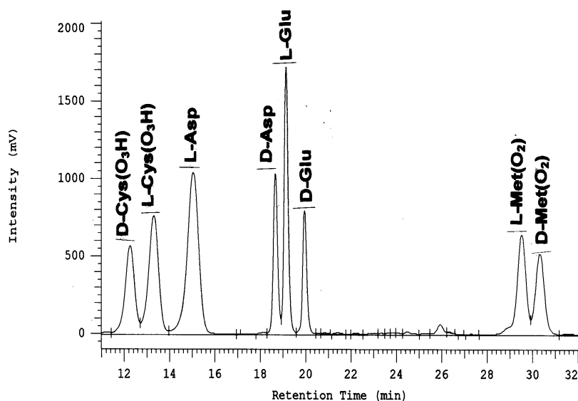
Figure 2. Separation of OPA-TATG derivatives of cysteic acid, asparatic acid, glutamic acid, and methionine-sulphon enantiomers, L-serine and L-histidine with PR-HPLC. (Resolution: D/L cysteic acid: 1.4; D/L methionine-sulphon: 1.3.)
