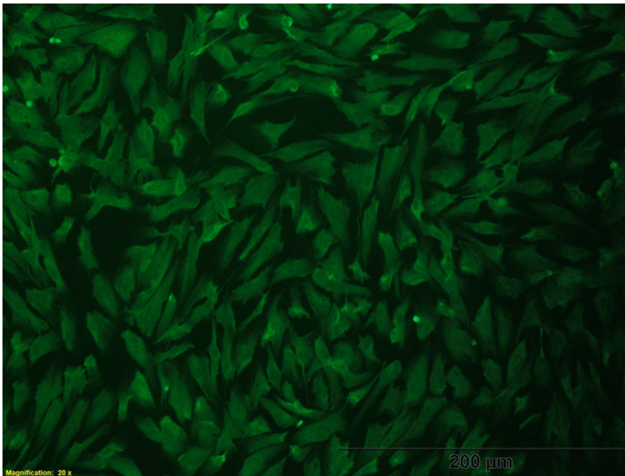
Fig 6. Fluorescent photomicrographs showing the presence of cytokeratin marker in BBdF-1 cells at) 20 \times Magnification
