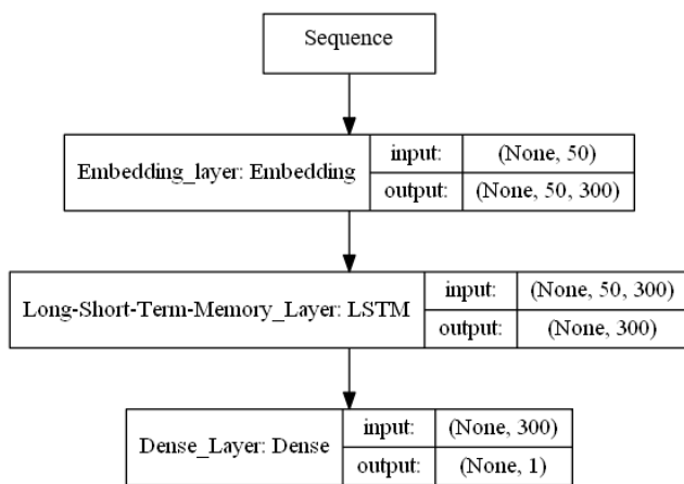
Fig. 1. NN architecture
