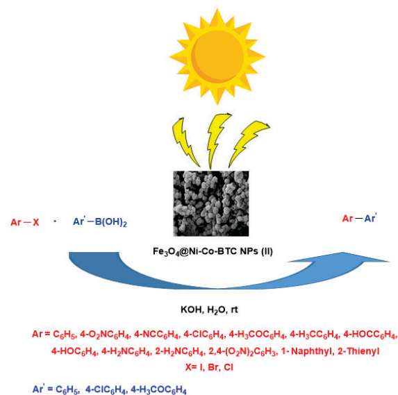
Scheme 2. Sun-light-driven Suzuki-Miyaura cross-coupling reaction of aryl halides and aryl boronic acids catalyzed by \text{Fe}_3\text{O}_4@ Ni-Co-BTC NPs (II)
