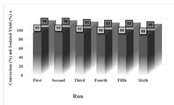
Figure 2. Reuse performance of \text{Fe}_3\text{O}_4@ Ni-Co-BTC NPs (II) in the sun-light-driven Suzuki-Miyaura cross-coupling reaction.
