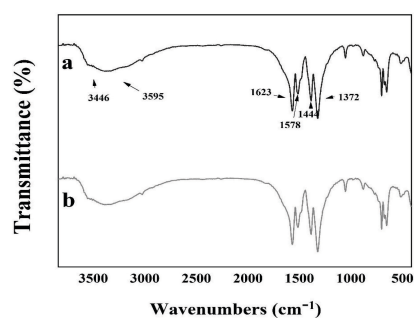
Figure 3. FT-IR spectra of \text{Fe}_3\text{O}_4@ Ni-Co-BTC NPs (II) (a) and the 6 th reused \text{Fe}_3\text{O}_4@ Ni-Co-BTC NPs (II) (b).
