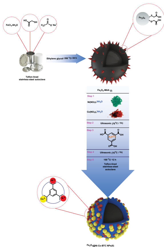
Scheme 1. Synthetic route to \text{Fe}_3\text{O}_4@ Ni-Co-BTC NPs (II).
