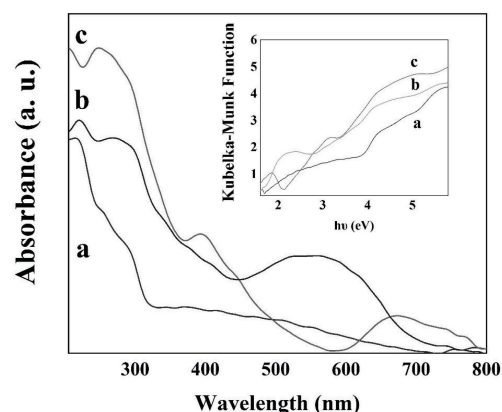
Figure 1. UV-vis. DRS spectra and Kubelka-Munk function (inset) of \text{Fe}_3\text{O}_4@Co\text{-BTC} NPs (a), \text{Fe}_3\text{O}_4@Ni\text{-Co-BTC} NPs (II) (b) and \text{Fe}_3\text{O}_4@Ni\text{-BTC} NPs (c).
