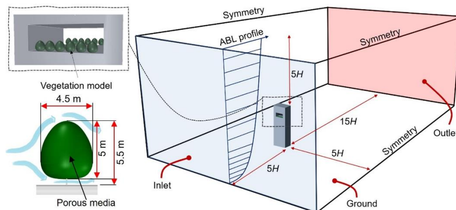
Figure 1. Computational domain and boundary conditions
