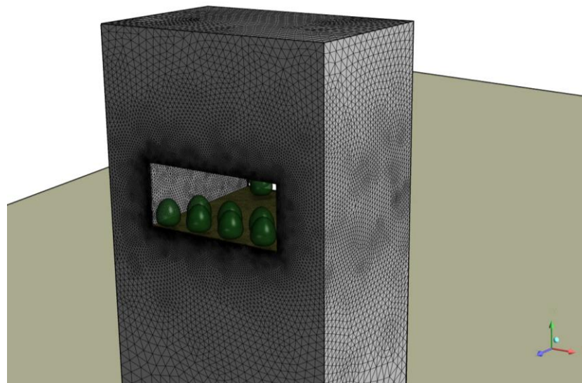
Figure 5. Computational mesh around the surfaces of the skygarden model highlighting refined areas
