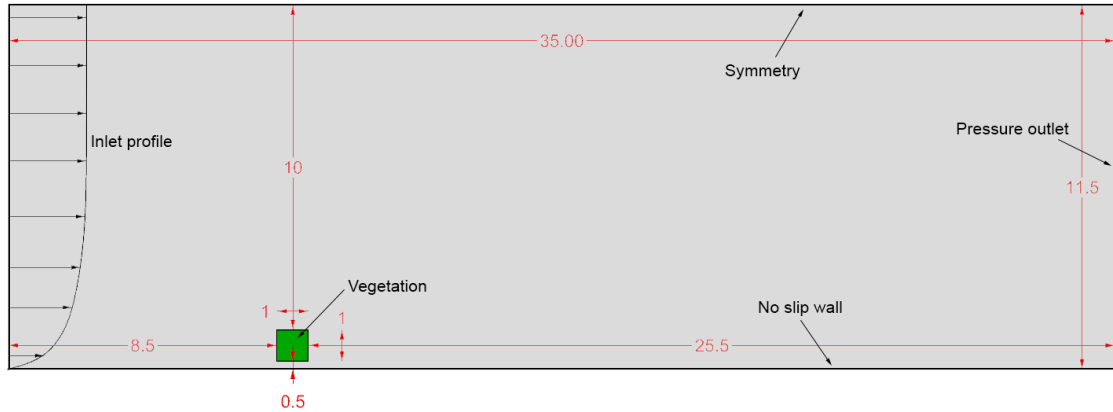
Figure 8. Simulation domain of the validation model, with the porous vegetation indicated by the green square and centred along the x-axis
