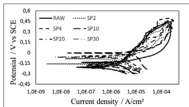
Figure 5 Cyclic polarization curves for different duration shot peening in 0,9 % NaCl
