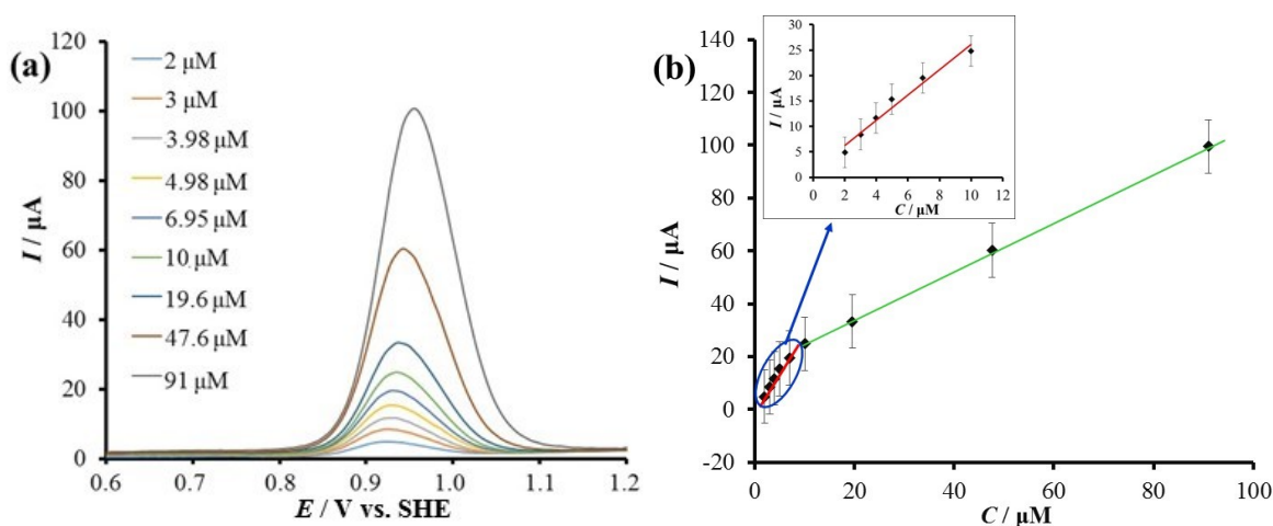
Figure 4. (a) Differential pulse voltammograms of BDD electrode for different concentrations of paracetamol in 0.3\text{ M H}_2\text{SO}_4 ; (b) current intensity calibration curve as a function of paracetamol concentration; T = 25\text{ }^\circ\text{C}
