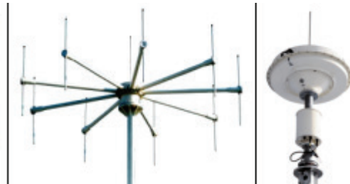
Figure 12. Coastal R&S DDF04E Maritime RDF with Shore and Ship Antenna – Source: R&S.
