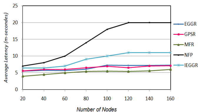
Fig. 10. End-to-end transmission delay.
