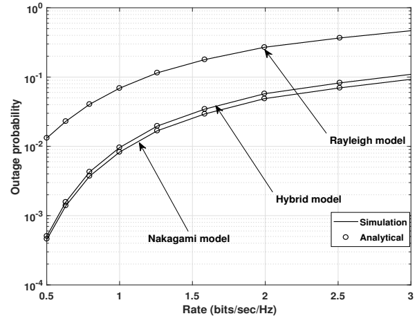
Fig. 8. Outage probability with respect to rate.
