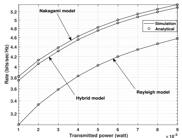
Fig. 12. Rate with respect to transmitted power.
