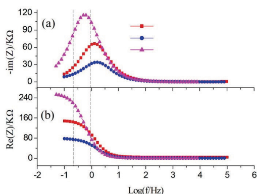
Figure 4. Variation of -Im(Z) (a) and Real(Z) (b) of MHDA modified gold electrode versus frequency for the applied potential E = -0.3\text{ V} . (▲) 1 h 15 min at \theta = 55^\circ\text{C} then for 1 h at \theta = 4^\circ\text{C} , (■) overnight at \theta = 4^\circ\text{C} and (●) \theta = 55^\circ\text{C} for 1 h 15 min.
