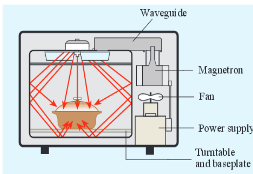
Fig. 3. Schematic diagram of a microwave oven (Hutcheon et al., 1992)
