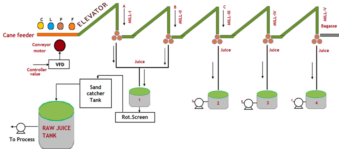
Figure 2. Schematic diagram for sugar cane crushing process.
