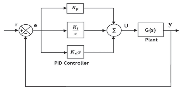
Figure 5. Closed loop system with PID controller.
