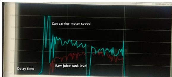
Figure 15. Real-time controller response with the proposed PID controller gain values.
