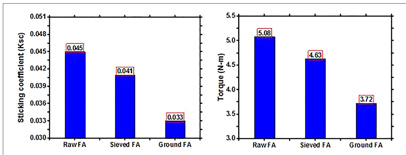
Figure 6. Comparative results of fly ash with different particle size on differential sticking tendency
