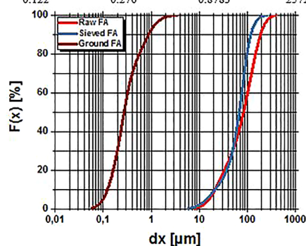
Figure 2. Particle size distributions of fly ashes
