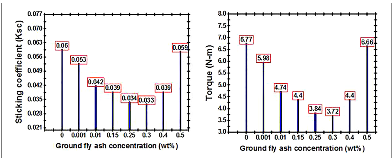
Figure 5. Effect of ground fly ash concentration on the sticking coefficient of drilling mud
