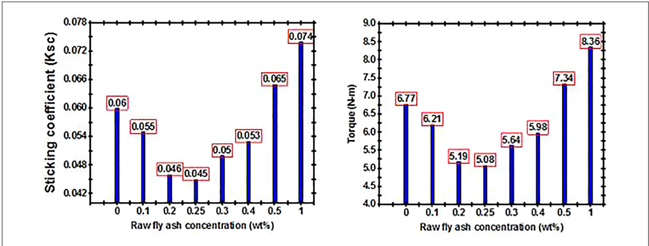
Figure 3. Effect of raw fly ash concentration on the sticking coefficient of drilling mud
