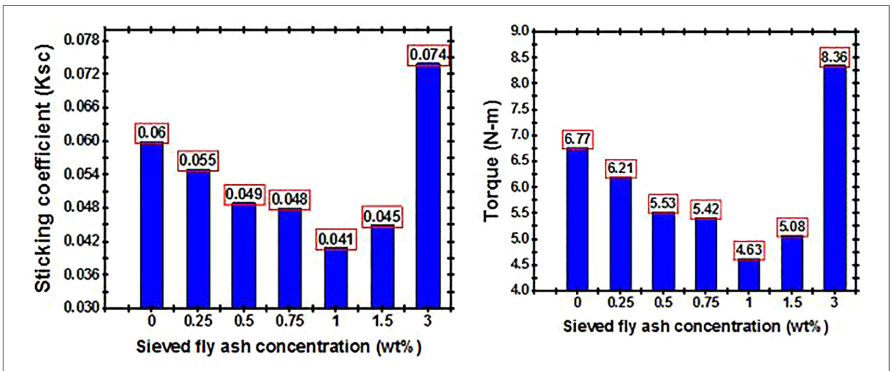
Figure 4. Effect of sieved fly ash concentration on the sticking coefficient of drilling mud
