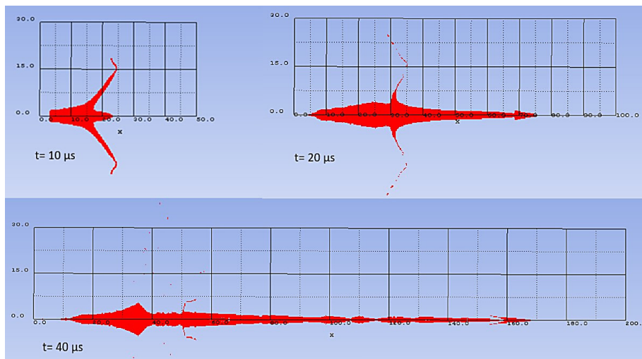
Figure 6: Shaped charge jet
