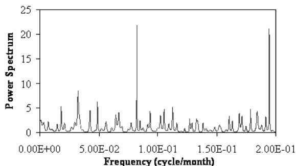
Figure 5. MEM power spectrum Atar rainfall (1923-2004).
