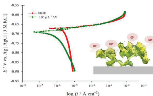
Spontaneous physisorption of Alchemilla vulgaris L. extract on aluminium surface.
